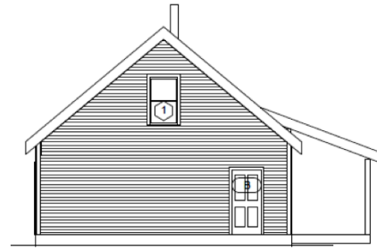
② SOUTH ELEVATION 1/8" = 1'-0"
